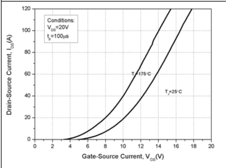
Transfer Characteristic
