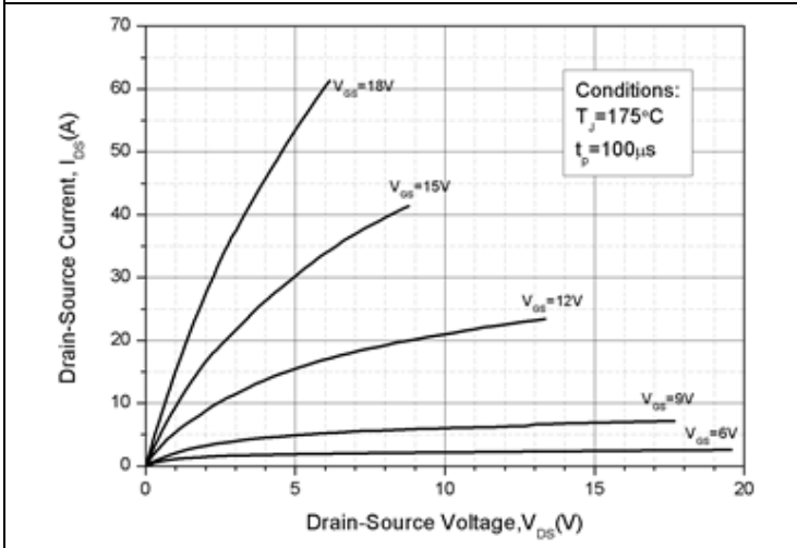
Output Characteristics T_J = 175\text{ }^\circ\text{C}
