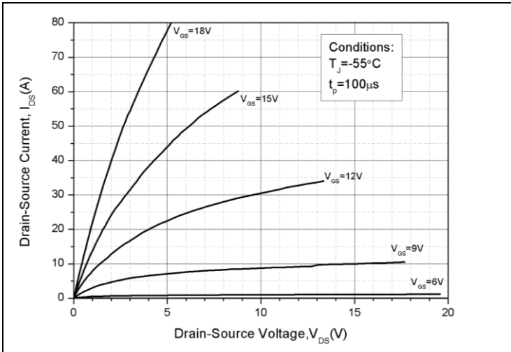
Output Characteristics T_J = -55\text{ }^\circ\text{C}
