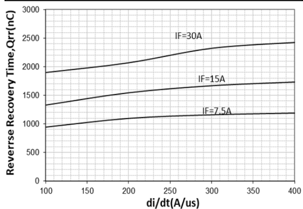
Fig.7 Reverse recovery charges versus di/dt
