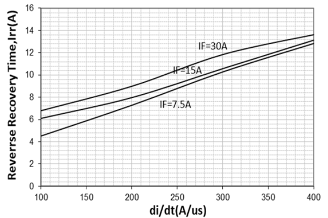
Fig.6 Peak reverse recovery current versus di/dt
