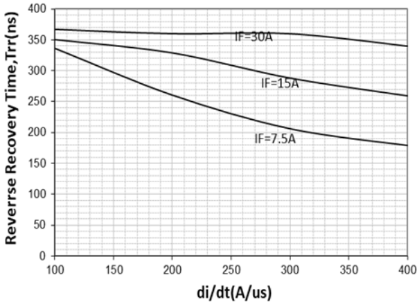
Fig.5 Reverse recovery time versus di/dt
